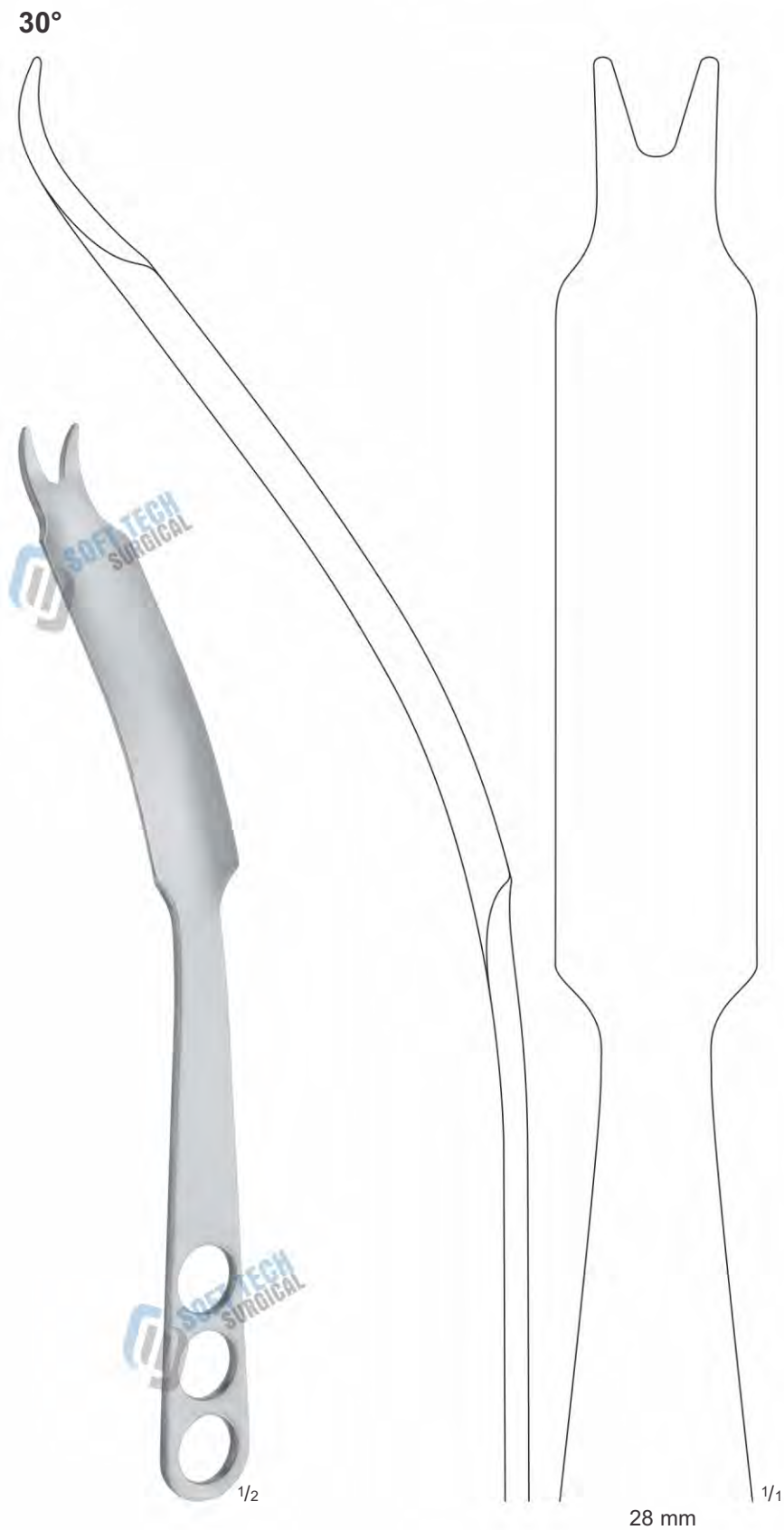
MIOS, HIP RETRACTOR 24-0430 V-tip 315 mm
