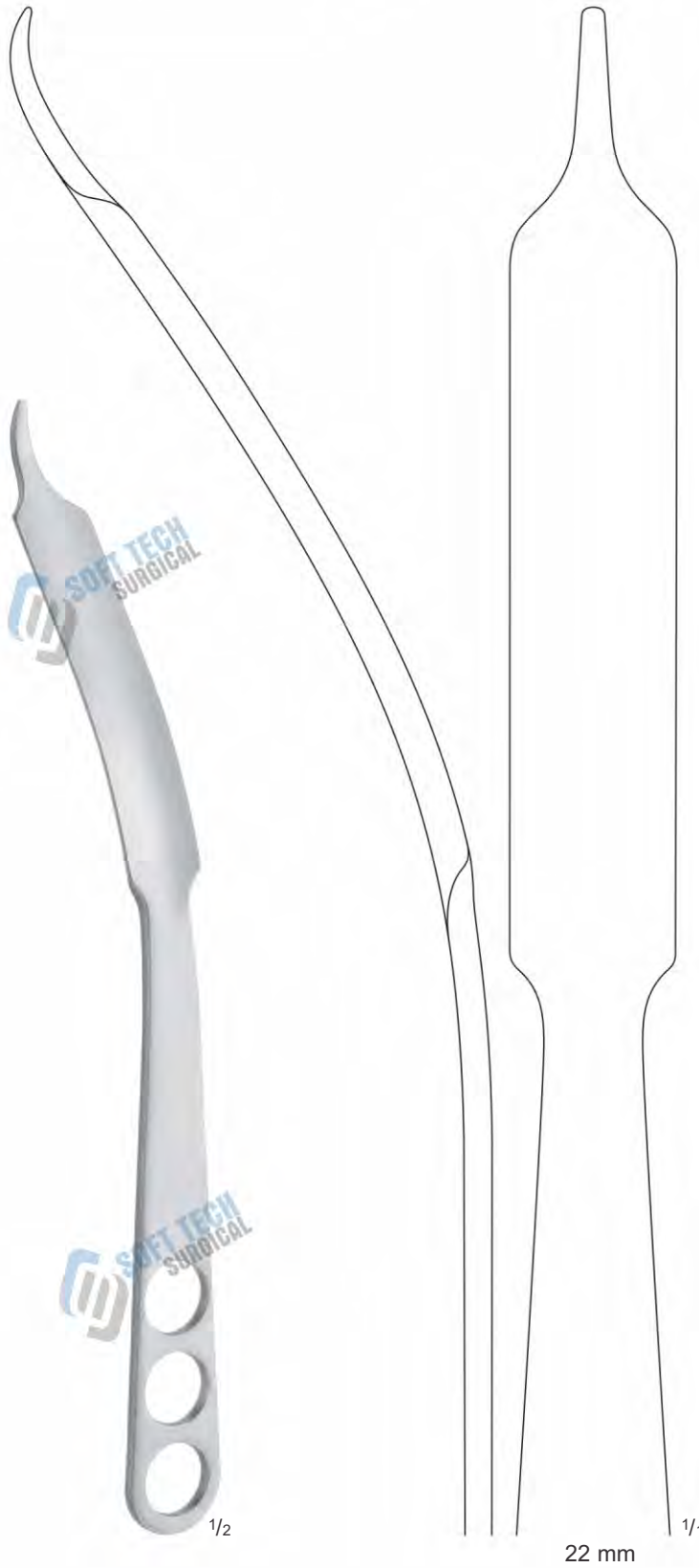
MIOS, HIP RETRACTOR 24-0425 sharp tip 315 mm
