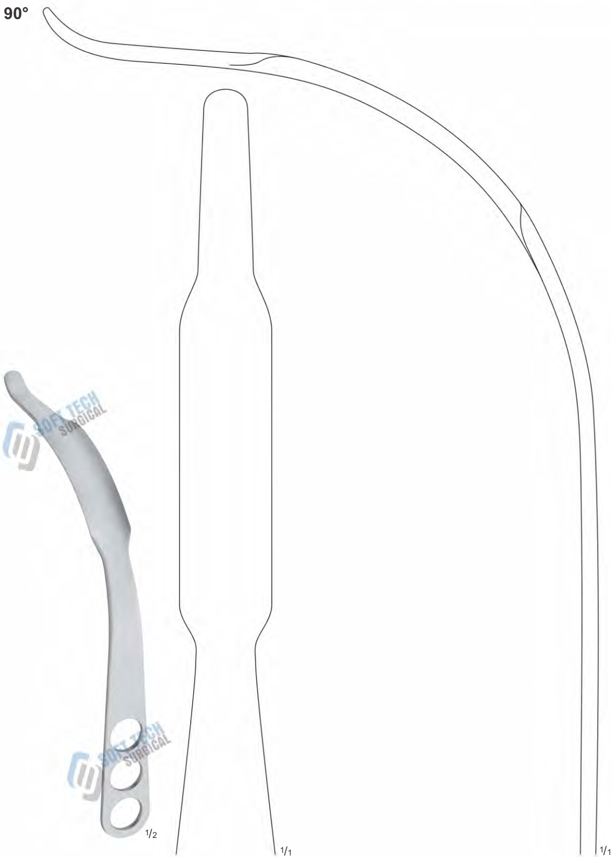
MIOS, FEMORAL NECK LEVER 24-0400 femoral neck tip 240 mm
