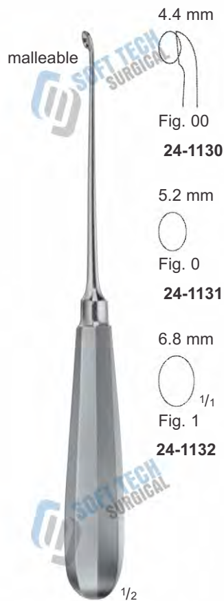
HALLE BONE CURETTES 215 mm
