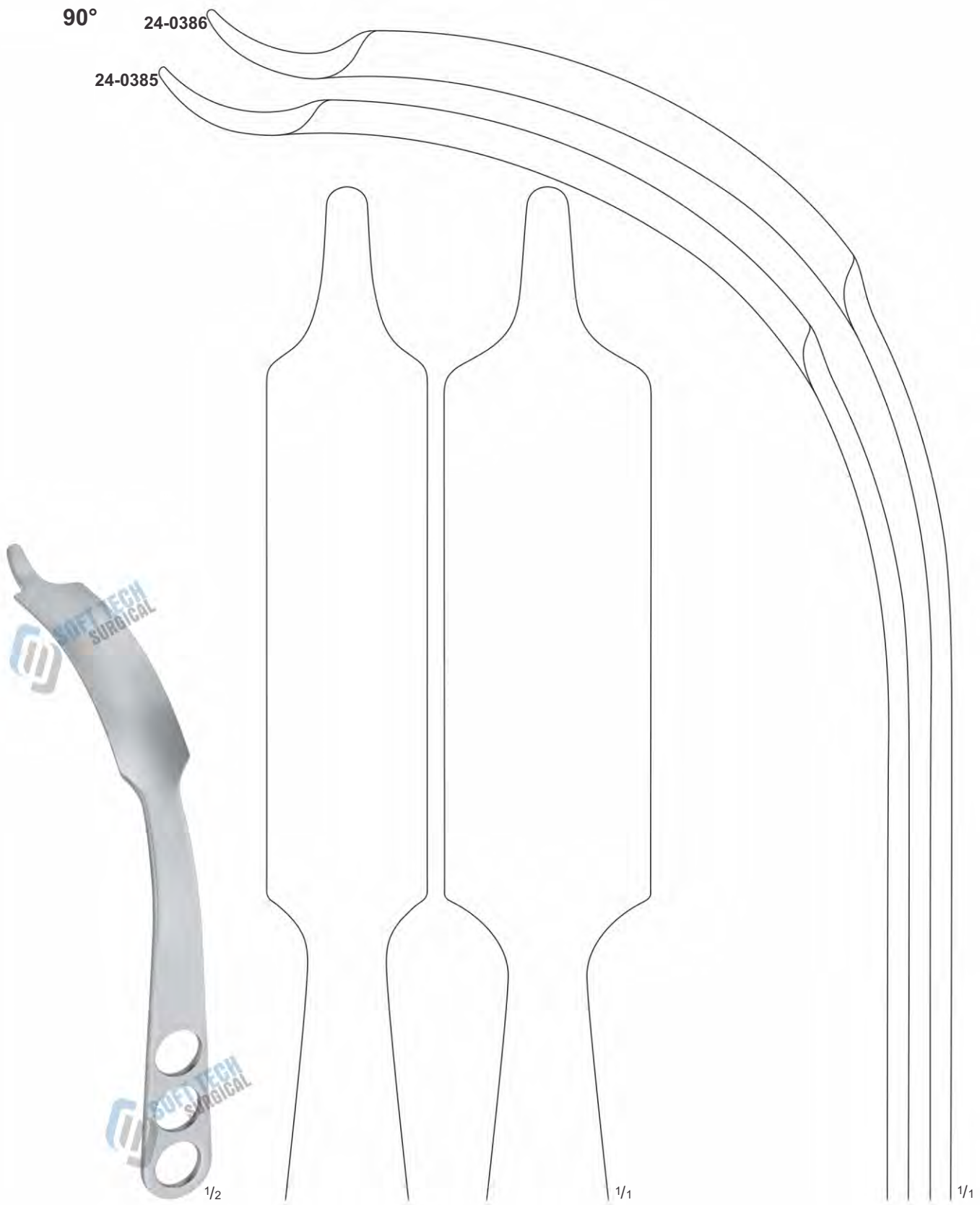
MIOS HIP RETRACTOR blunt tip 240 mm
